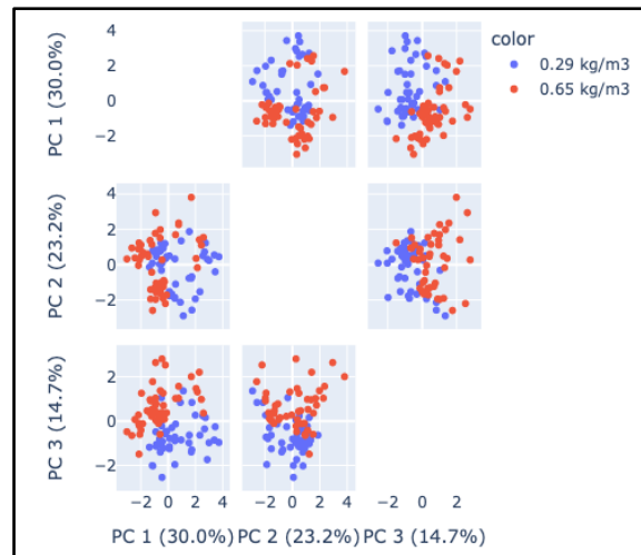
Figure 2. Results of PCA for a single section with good separation between two classes of target variable (volume of the explosives). For better resolution only first three PC are shown (resolving > 67% of variance). Colours are corresponding to the total volume of explosives per m 3 of the excavation.
